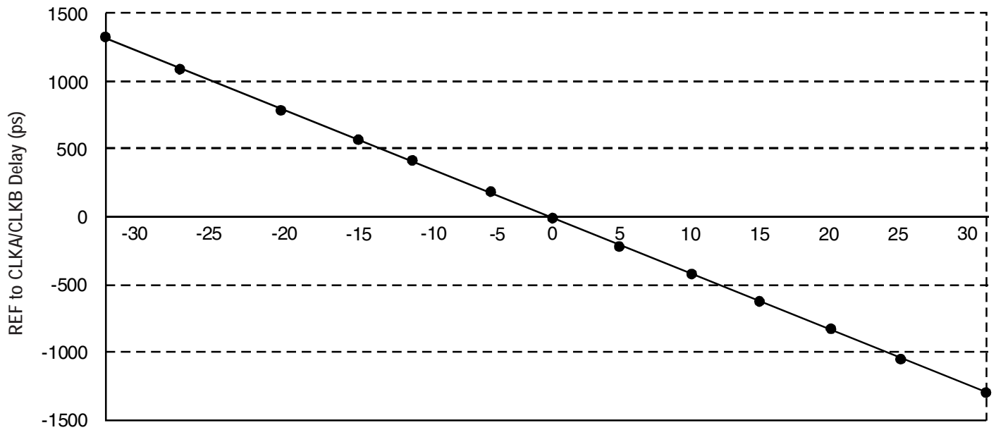
OUTPUT LOAD DIFFERENCE BETWEEN FBK PIN AND CLKA/CLKB PINS ( pF)
